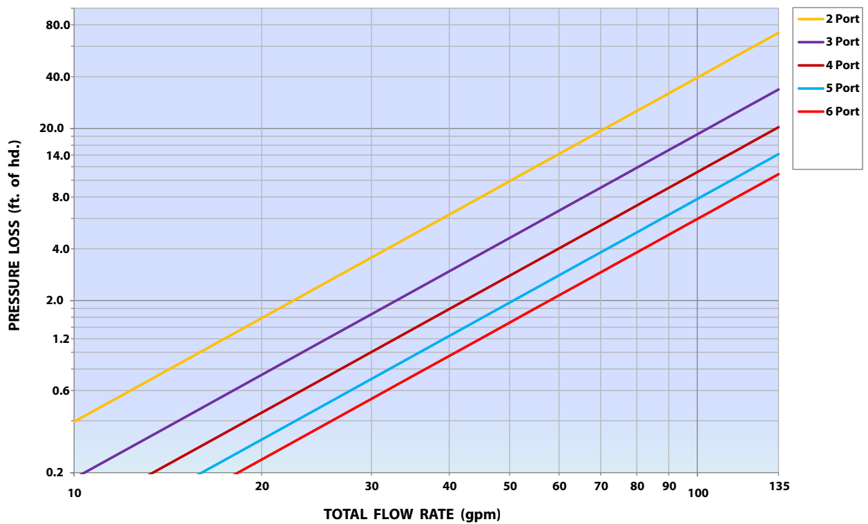
M-8228 High Capacity Manifold (2") FLOW CHART
