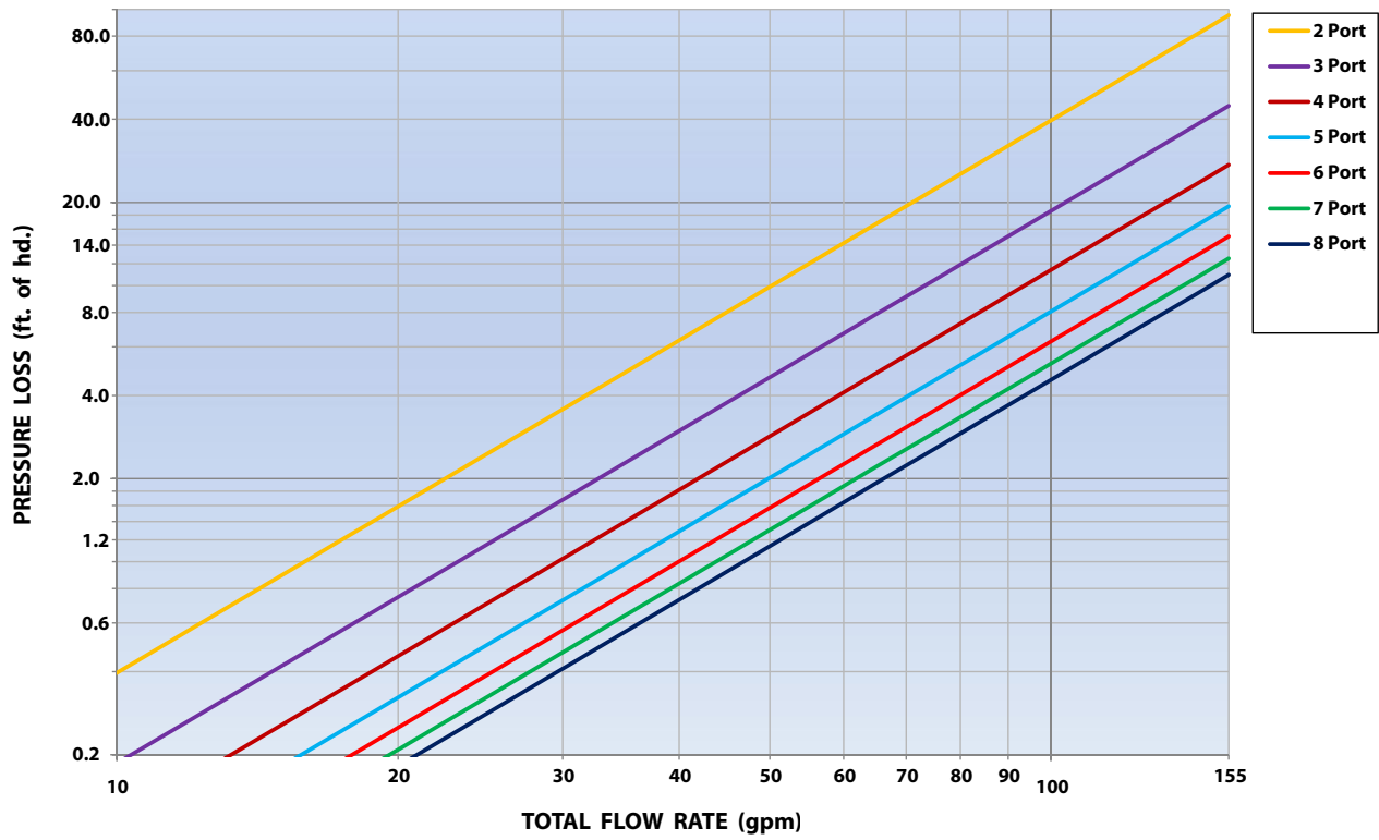
M-8220 High Capacity Manifold (1/2") FLOW CHART
