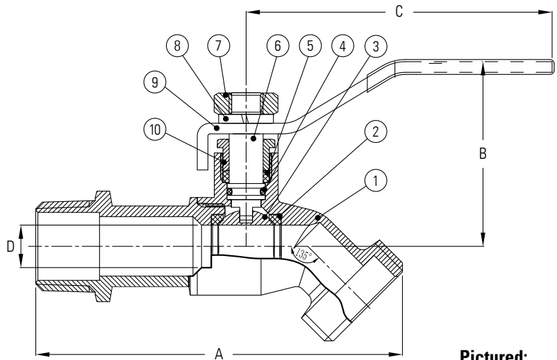
Pictured: T-537CP Cut-away
